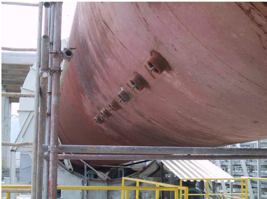
Cardox Sockets mounted onto rotary kiln. Sockets positioned 3 rows around diameter of kiln spaced @ 0.75m.
